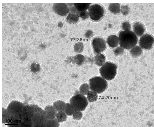
Fig. 3 TEM micrographs of \text{Ba}_3\text{Gd}_{0.93}\text{Tb}_{0.07}\text{P}_3\text{O}_{12} powder calcined at 1100 °C
