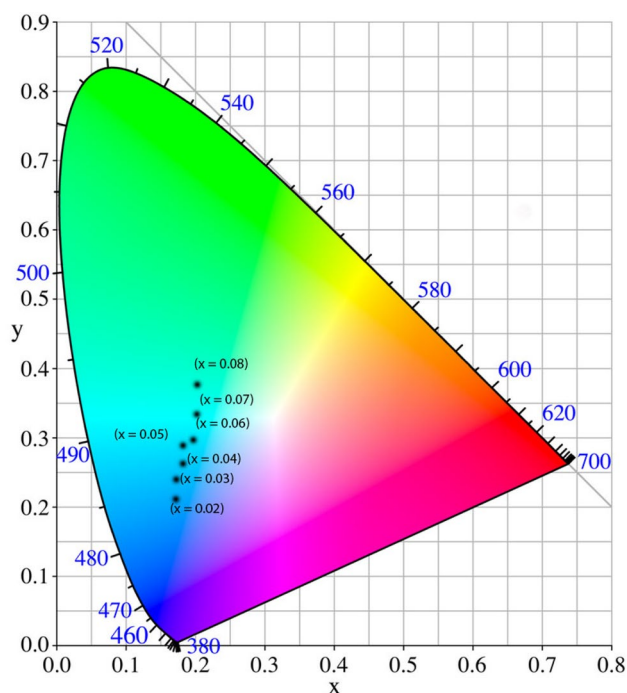
Fig. 12 CIE chromaticity diagram for \text{Ba}_3\text{Gd}_{1-x}\text{Tb}_x\text{P}_3\text{O}_{12} ( x=0.02 – 0.08 ) nanophosphors
