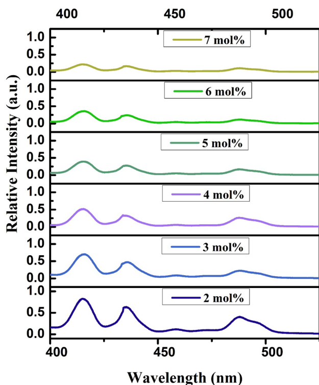
Fig. 8 Normalized Emission spectrum of \text{Ba}_3\text{Gd}_{1-x}\text{Tb}_x\text{P}_3\text{O}_{12} ( x=0.02-0.07 ) nanophosphor scrutinized at \lambda_{\text{ex}}=224 nm (Color figure online)
